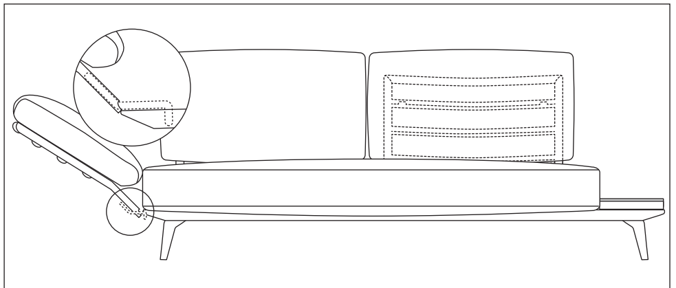
24: Components used for the above: King Cove 2 Seater with Shelf & Sun Lounge Brackets: 1x Platform (with 4x Legs); 1x Seat Cushion; 3x Back Frames; 3x Back Cushions; 4x Back Brackets; 2x Sun Lounge Brackets; 1x Shelf Frame; 1x Shelf Insert.
