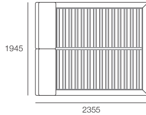
Bed Head and Base Top View (No Mattress)
